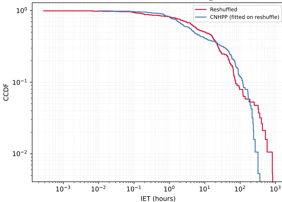
User 1992063859 - Reshuffled vs CNHPP A_{\text{fit}}=0.6262
